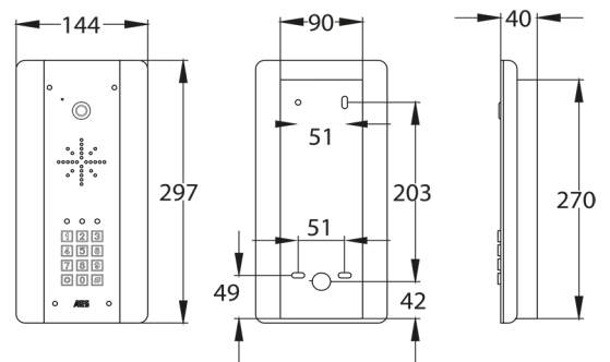
SLIM - ARCHITECTURAL WITH KP
