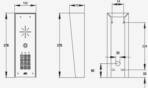
SLIM - IMPERIAL WITH KP
