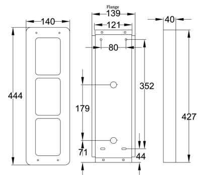
MULTI-LITE-FBPK-EU (Flush)
